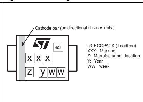
Figure 12. Marking information
